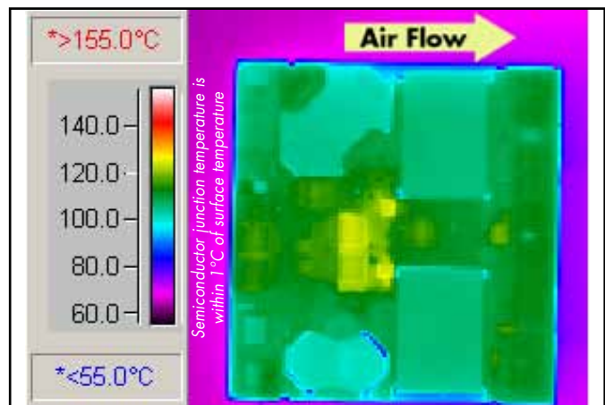
Figure 6: Thermal plot of converter at 59 amp load current with 55°C air flowing at the rate of 200 LFM. Air is flowing across the converter from input to output (nominal input voltage).
