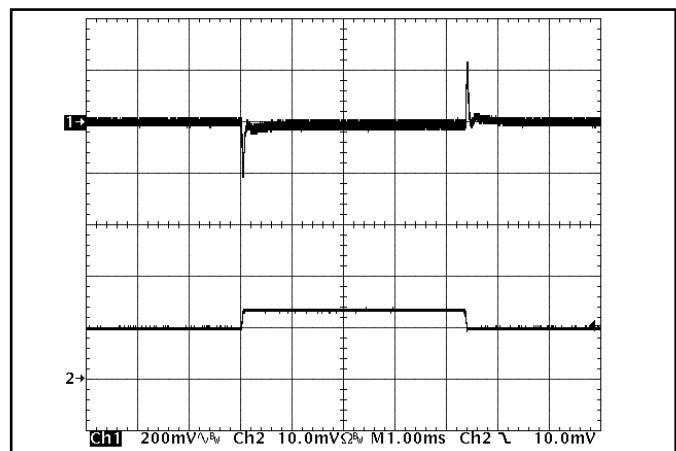
Figure 12: Output voltage response to step-change in load current (50%-75%-50% of I out (max); dI/dt = 5A/μs). Load cap: 480μF, 15 mΩ ESR tantalum cap and 1μF ceramic cap. Top trace: V out (200mV/div), Bottom trace: I out (50A/div).
