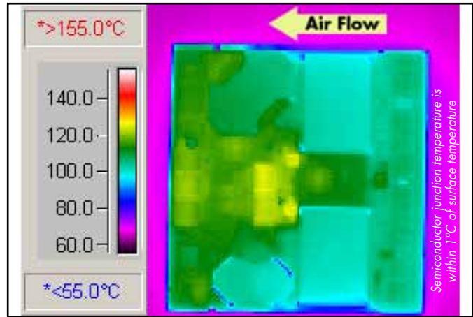
Figure 8: Thermal plot of converter at 58 amp load current with 55°C air flowing at the rate of 200 LFM. Air is flowing across the converter from output to input (nominal input voltage).
